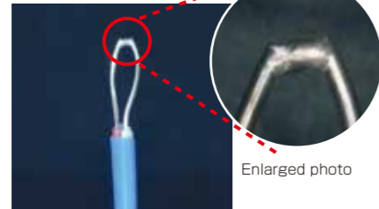
Diameter of thermocouple: 0.3 mm Welding condition: Welding current set to 2A
